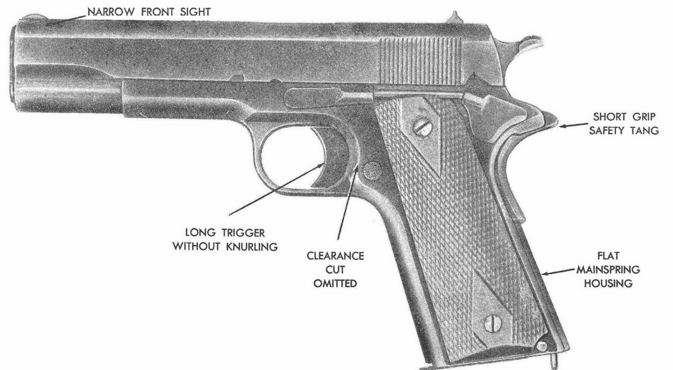
Left side of pistol M1911—showing exterior difference between pistol M1911 and M1911A1
