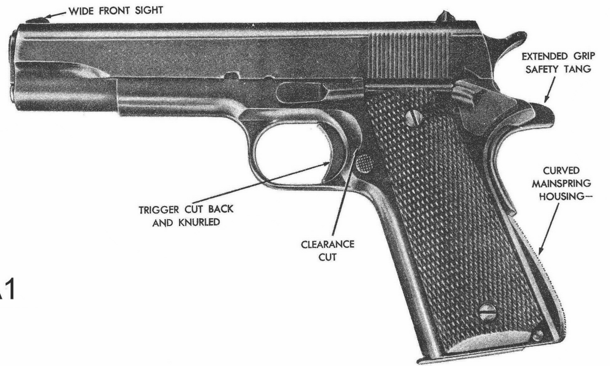
Left side of pistol M1911A1—showing exterior difference between pistol M1911 and M1911A1.
